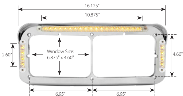
Front view 87593
